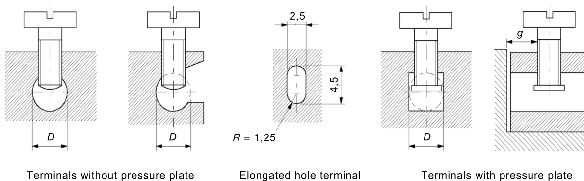
Figure 1 – Pillar terminals
