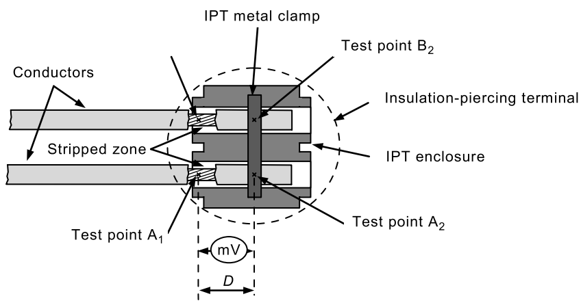
Figure D.1 – Example of insulation-piercing terminals
