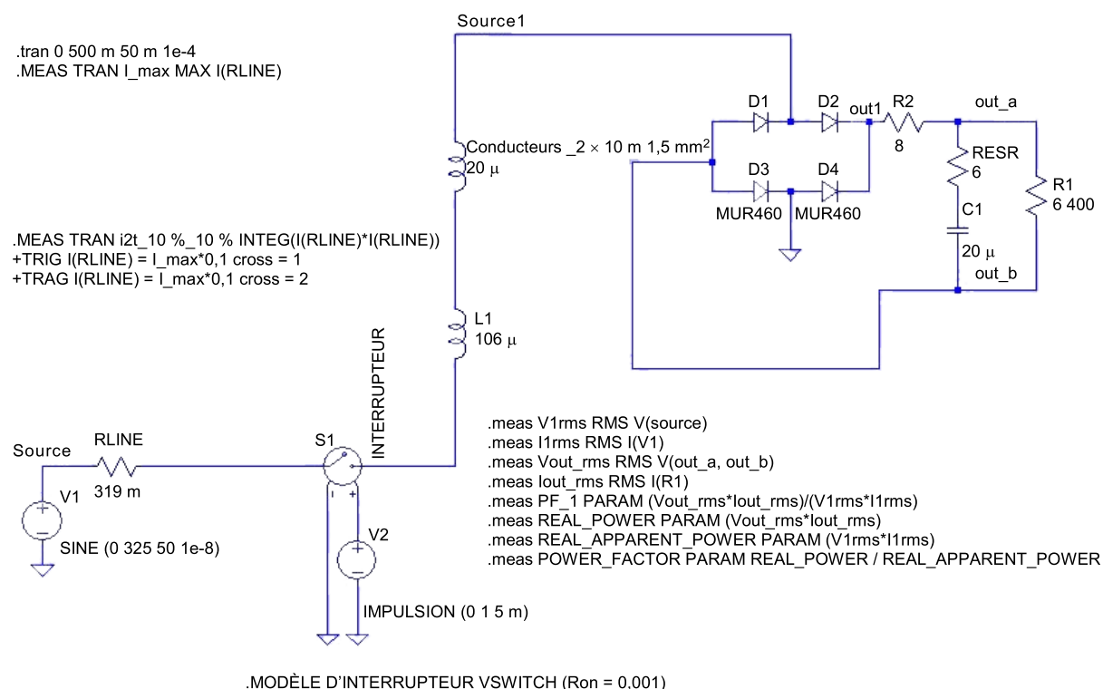
Figure C.2 – 230 V 15 W (modèle LT spice)
