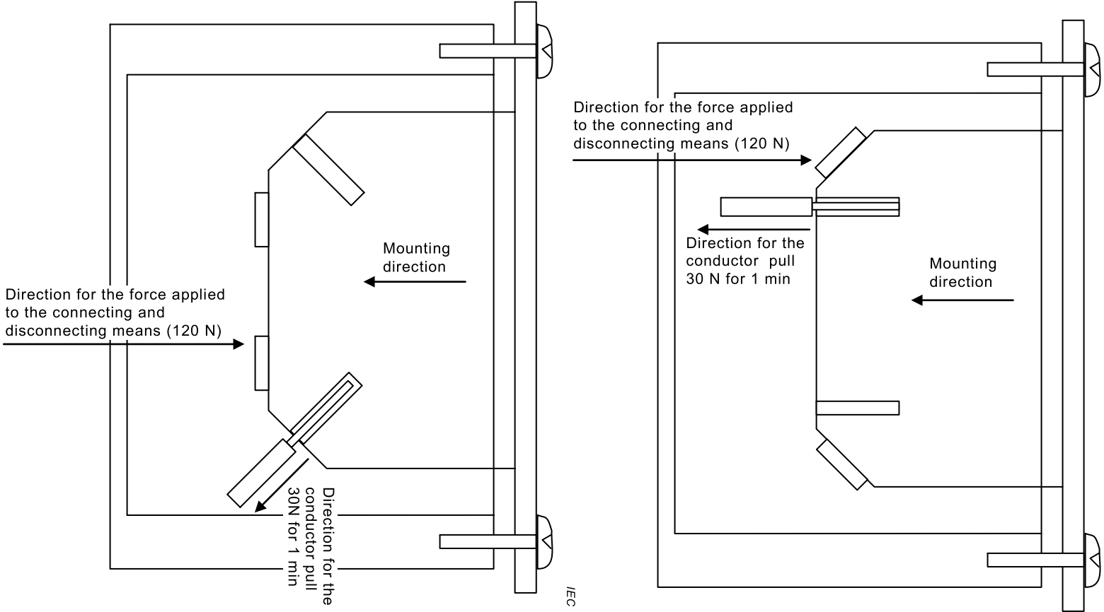
Figure 22a – Determination of the direction of the forces to be applied
