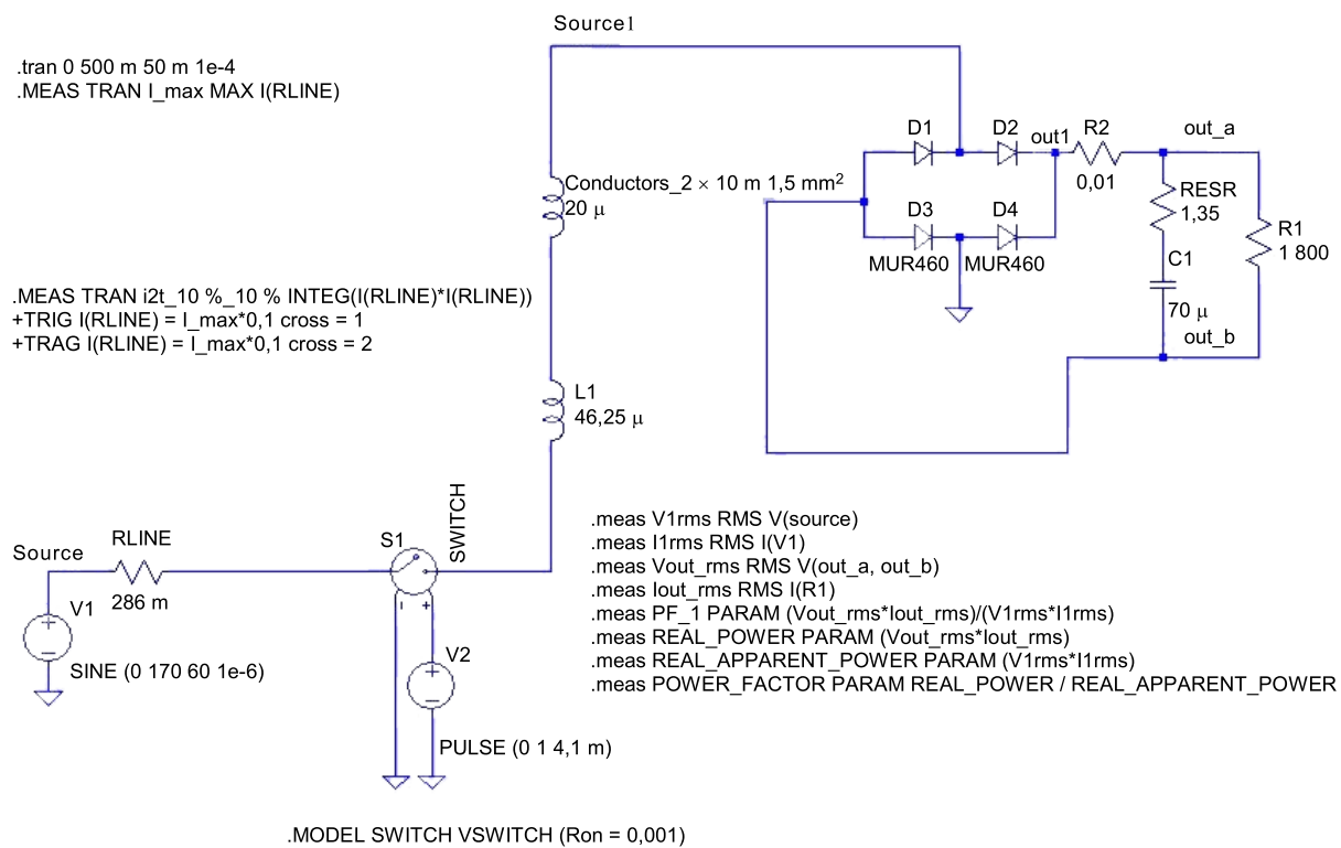
Figure C.1 – 120 V 15 W (LT spice model)
