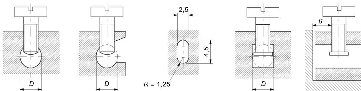
Bornes sans plaquette
