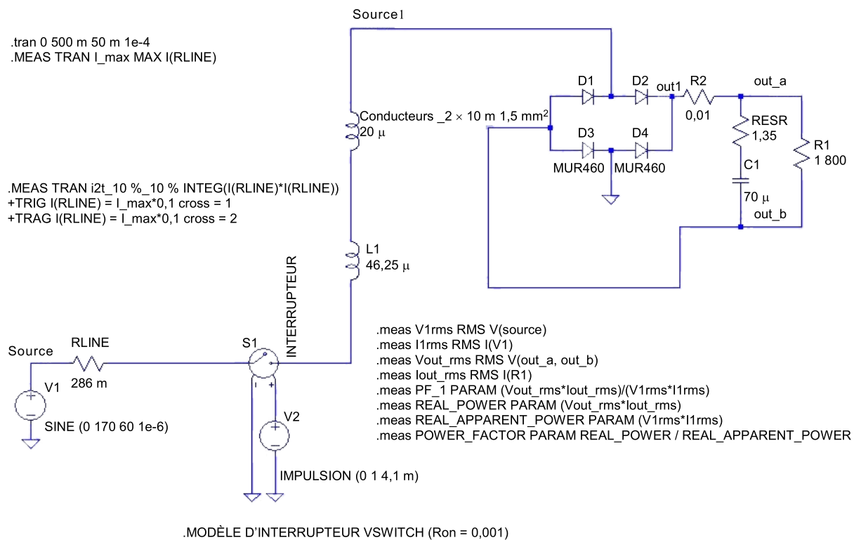
Figure C.1 – 120 V 15 W (modèle LT spice)
