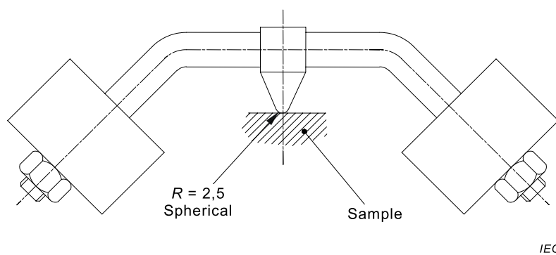
Figure 19 – Ball-pressure apparatus
