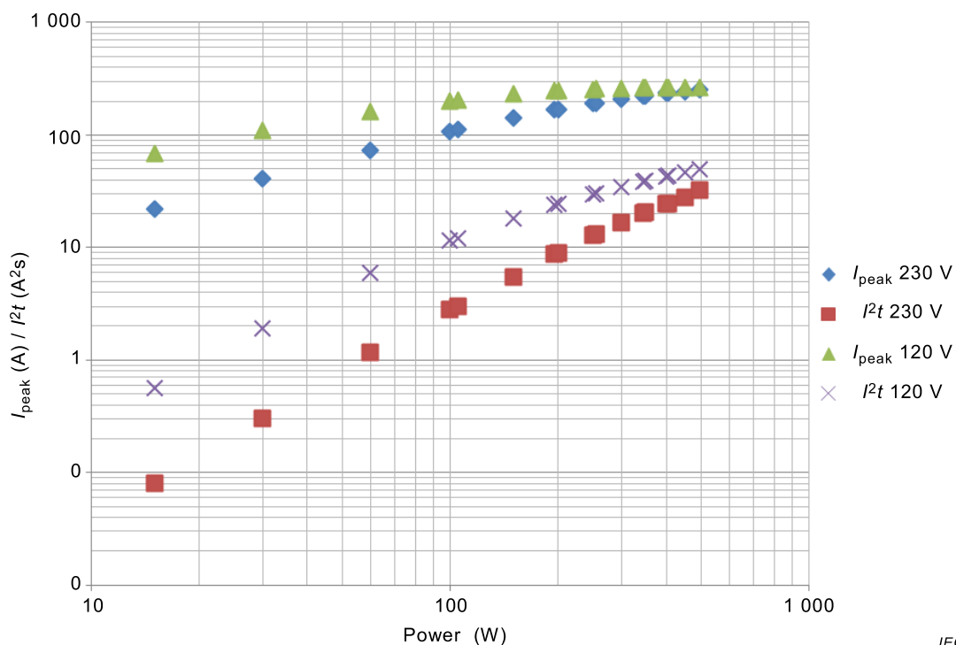
Figure C.4 – I_{\text{peak}} and I^2t for multiple lamp loads
